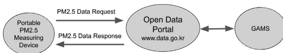
Fig. 4. PM 2.5 data fetch using HTTP protocol from the open data portal www.data.go.kr connected to GAMSSs in Korea. GAMSS, government-authorized PM monitoring station; HTTP, Hypertext Transfer Protocol; PM, particulate matter.
