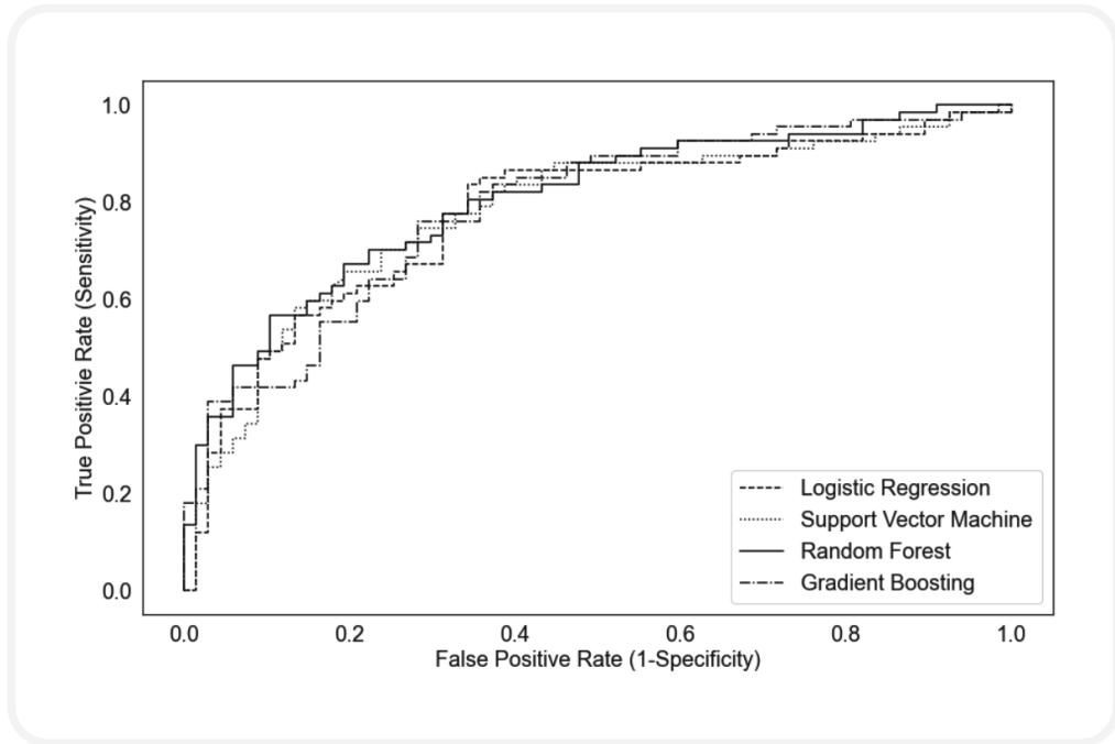
Fig. 1. ROC Curve
