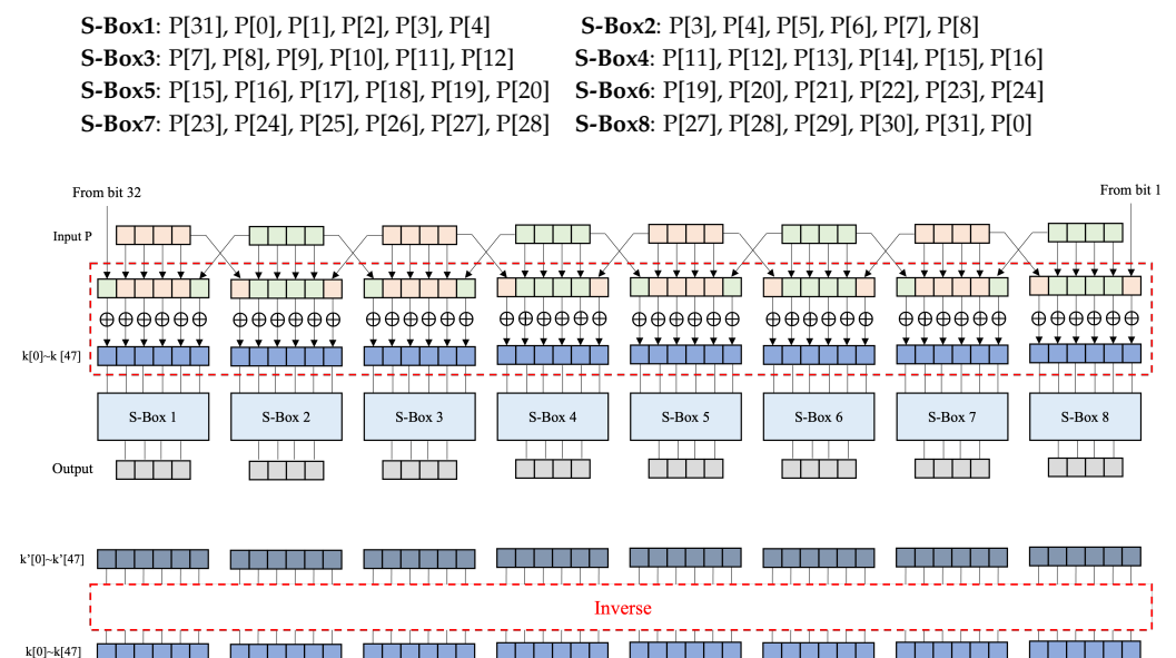
Figure 5. The Type A expansion P-Box: Each 32-bit input P is divided into eight 4-bit blocks. The blocks at both ends are used to XOR with the key k from both sides k \leftarrow \text{CNOT}(k, P) . Since the XOR result is stored in the key k , P remains unaffected and can be reused. The modified key k' is then used in the S-Box to obtain the output. Finally, k' is processed by inverting the operations in the red-dotted box to restore the original key k .
